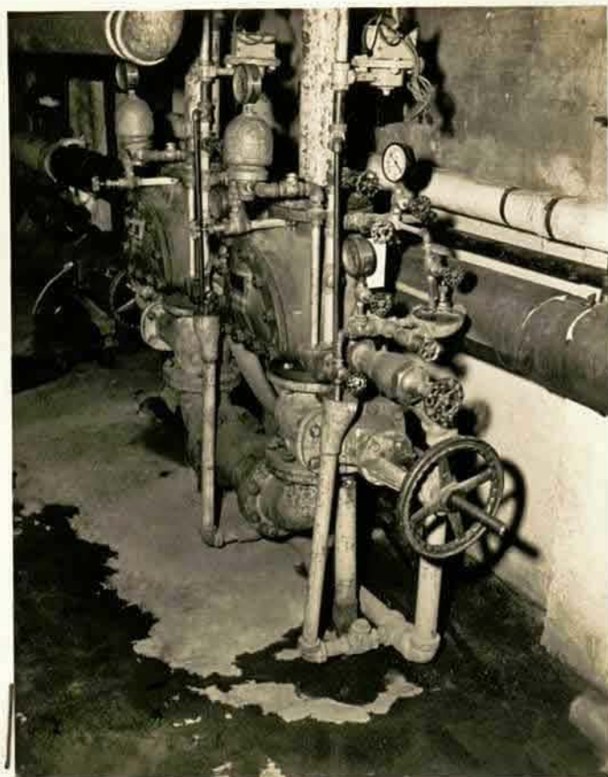
Neg. No. DB 7847 Dispo: L HQ Dest Photo's Manuel Dept. FIRE HALL Caption FIRE SPRINK- LER SYSTEM IN HMC COMMUNICATION SCHOOL.
