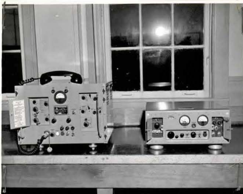
HMCS CORNWALLIS DB 12902 L Porter Comm School 27-8-59 Comm. Equipment Left:-TED3 Transmitter Right:-URR35 Receiver.
