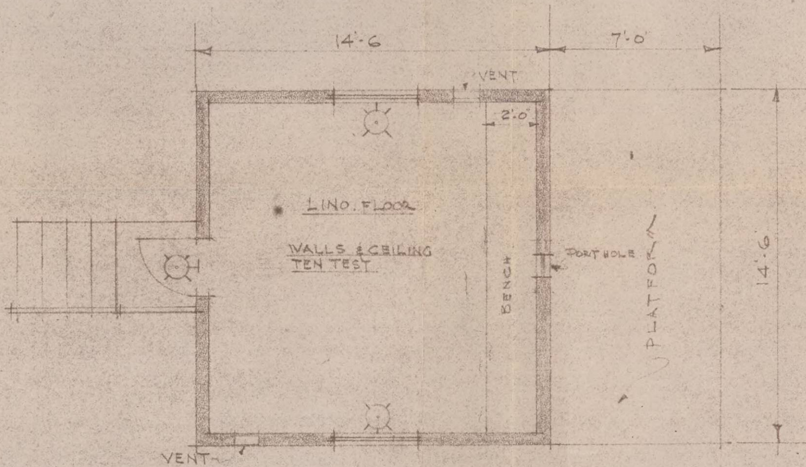
FLOOR PLAN
